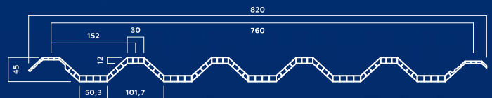
Drawing - Twin Wall OD 760
