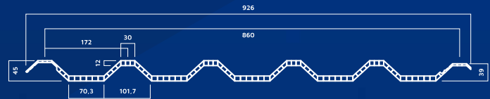
Drawing - Twin Wall OD 860
