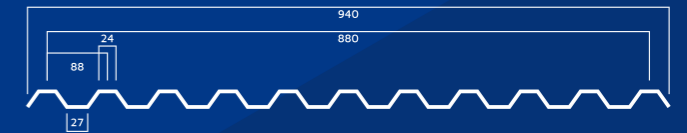
Drawing - Single Wall OD 880 Greca
