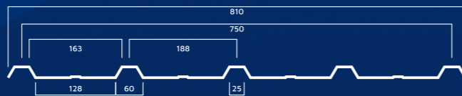
Drawing - Single Wall OD 750 Trimdeck
