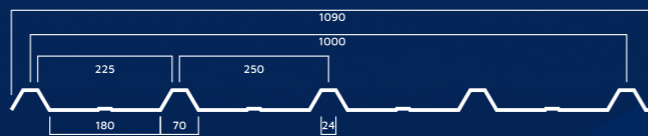
Drawing - Single Wall OD 1000 Trimdeck
